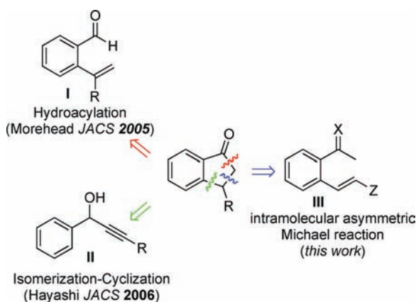
Scheme 1. Methods for the Asymmetric Construction of the Indanone Ring
