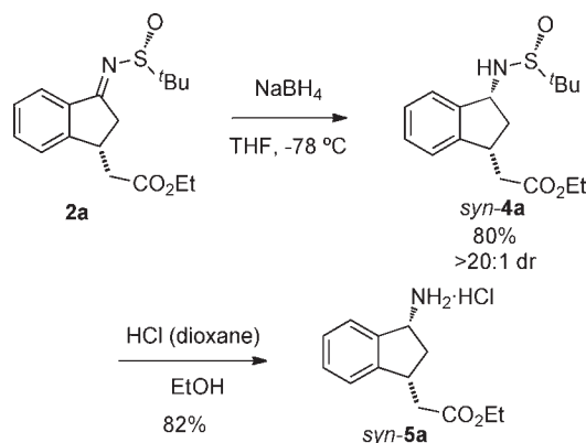
Scheme 4. Chemoselective Reduction Leading to \delta -Amino Acid Derivatives
